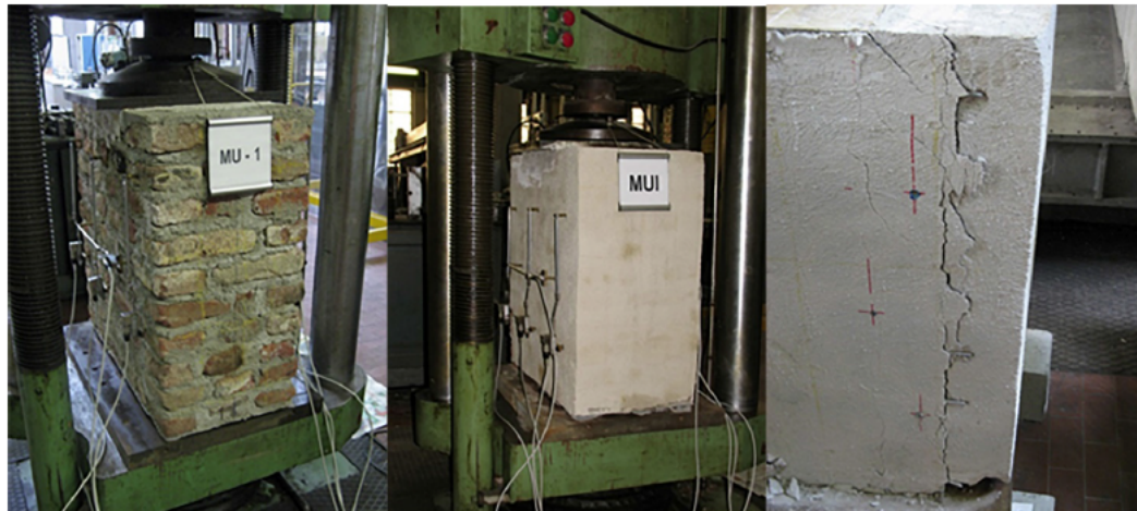
Figure 7: Compression test of: (a) original masonry specimens (MU); (b) masonry specimens strengthened by injection technique (MUI); (c) masonry specimens strengthened by jacketing wall technique (RMA).
