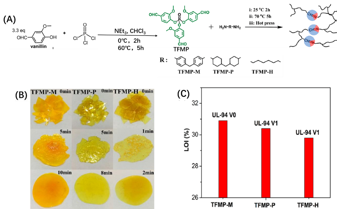
Figure 7: (A) Synthetic Route of TFMP and preparation of Schiff Base CANs, (B) Reprocess of Schiff base CANs at different times at 180°C under 15 MPa pressure, and (C) LOI and UL-94 rating of CANs. Adapted with permission from ref. [91]. Copyright 2018 American Chemical Society.
