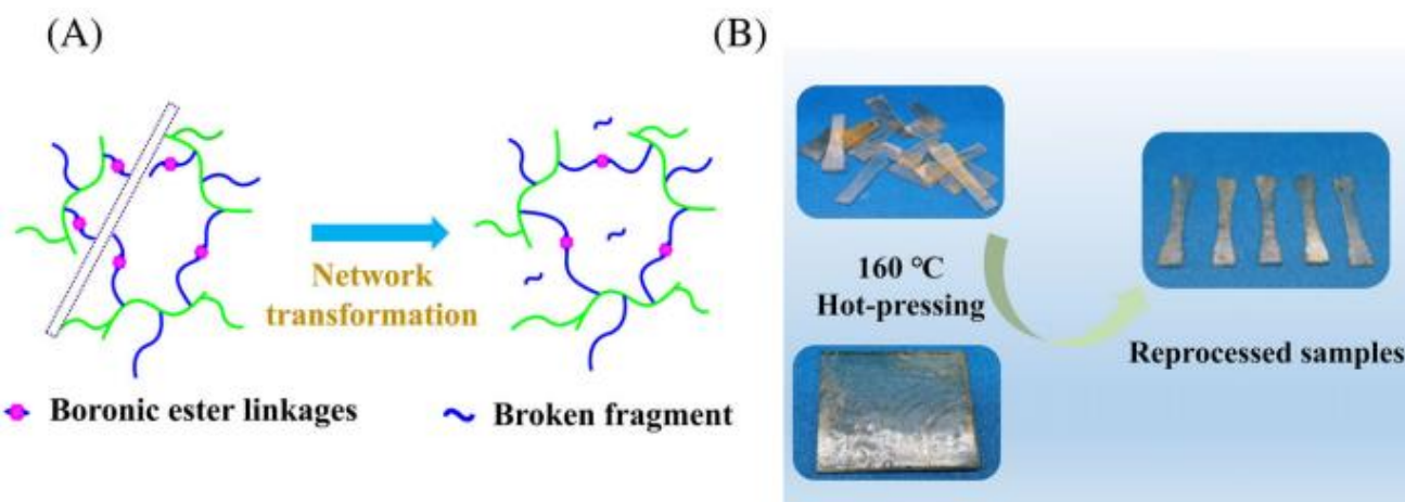
Figure 4: (A) The repair mechanism based on the boronic ester linkages; (B) The reprocessability ability of sample at 160 ^{\circ}\text{C} . Adapted with permission from ref.
