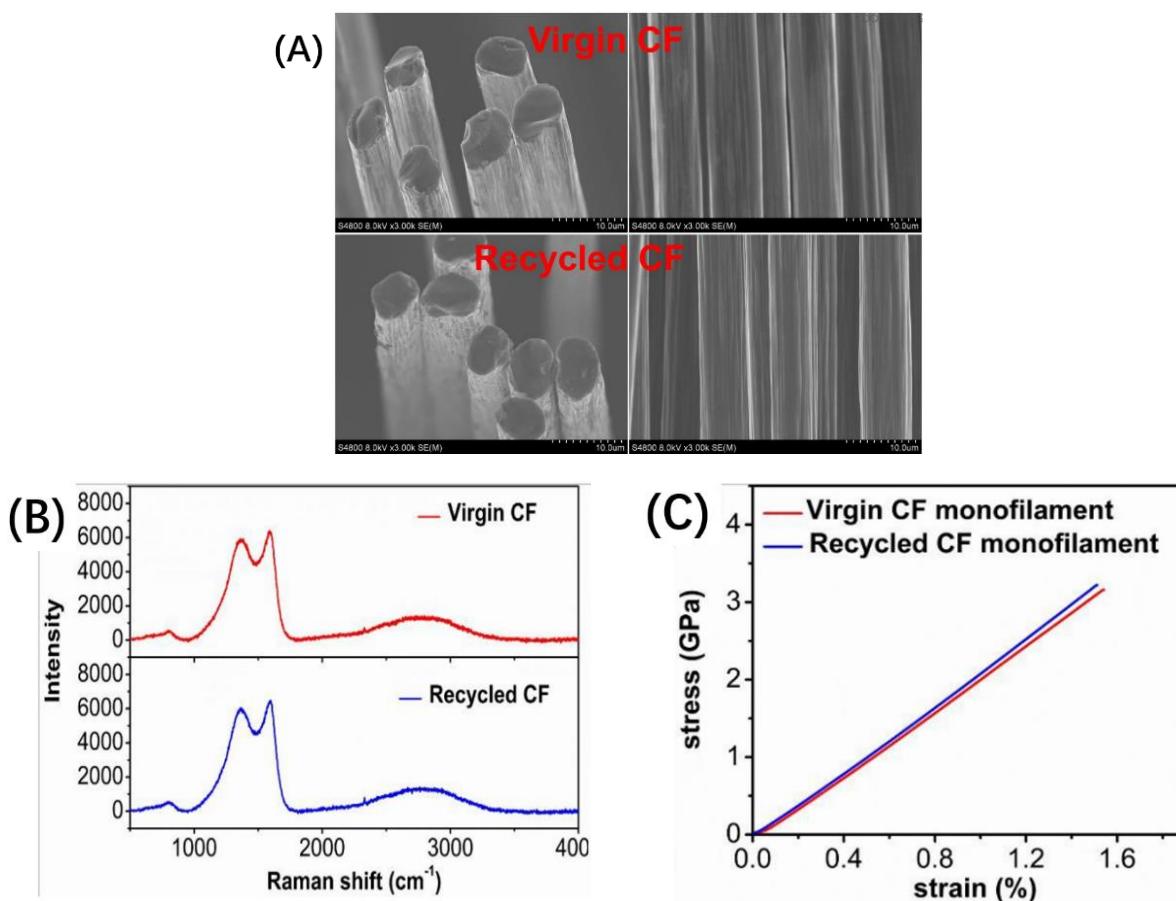
Figure 9: (a) The surface morphology of the virgin and recycled CF; (b) Raman spectra of the virgin and recycled CFs; (c) representative tensile stress-strain curves of the virgin and recycled CF monofilaments. Adapted with permission from ref. [80]. Copyright 2019 The Royal Society of Chemistry.
