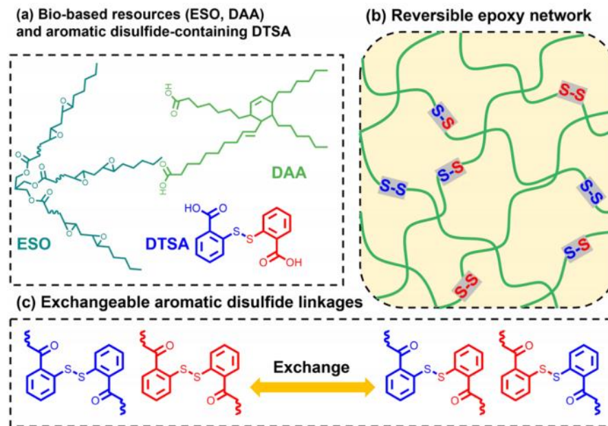
Scheme 16: (a) Chemical reagents of the epoxy network included epoxidized soybean oil (ESO), dimer aliphatic acid (DAA), and aromatic disulfide-containing agent (DTSA). Both ESO and DAA are bio-based resources containing long saturated or unsaturated fatty acid chains. The obtained reversible epoxy network (b) contains exchangeable aromatic disulfide linkages (c) which constantly break and reform.
