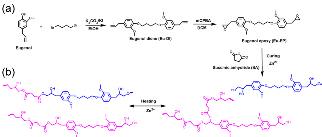
Scheme 5: (a) Synthetic Route of Eugenol Epoxy (Eu-EP); (b) Curing Reaction of Eu-EP and SA and illustration of Heat Induced Transesterification Reactions (TERs) in the Presence of Zinc Catalyst.
