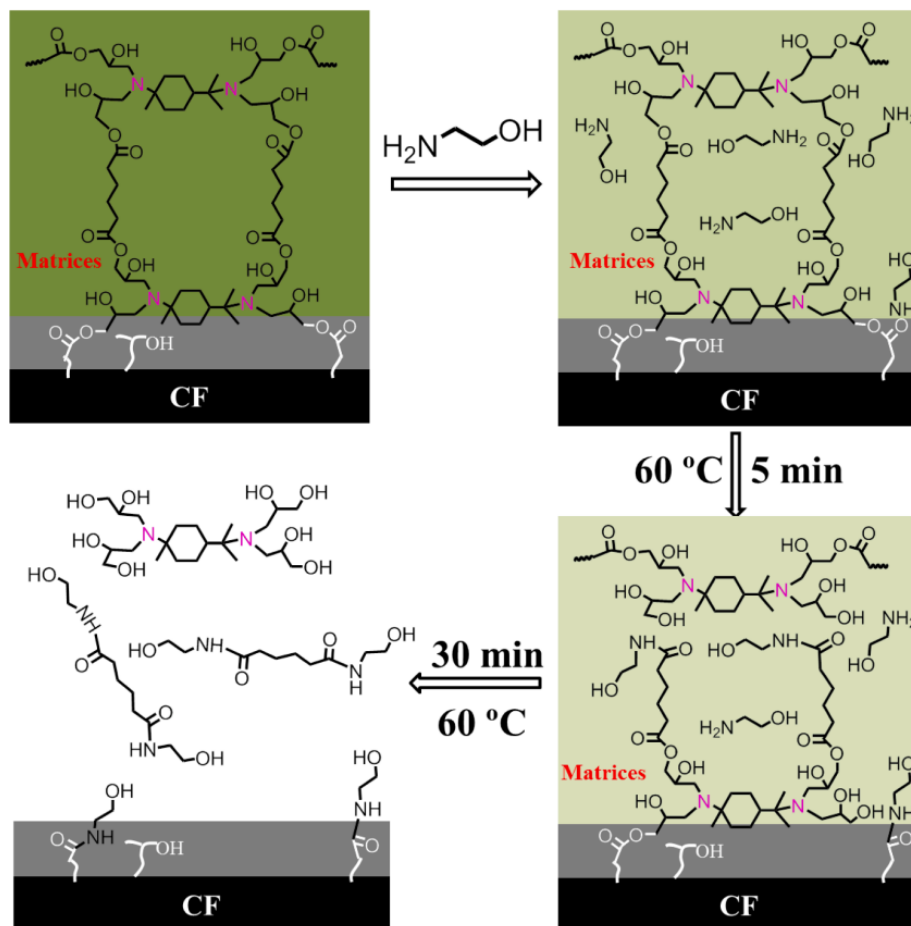
Scheme 7: Degradation mechanism of the EMDA-AA-CF composites in EA at 60 °C.
