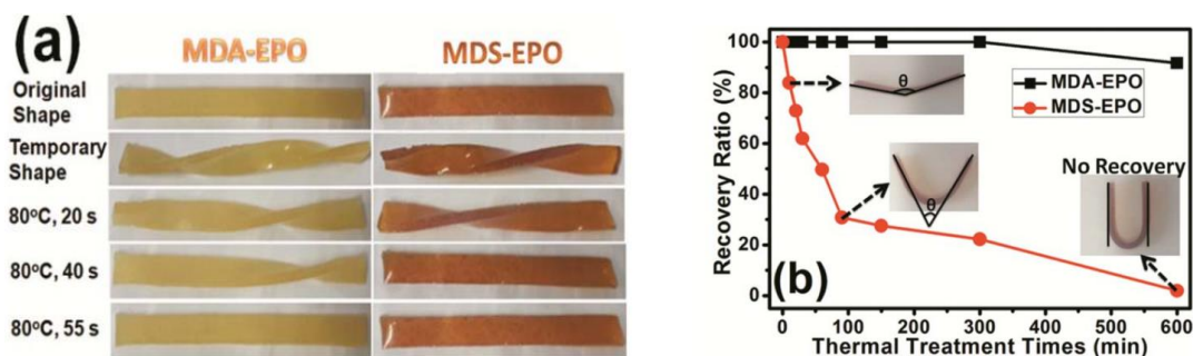
Figure 11: (a) Shape-memory effect of MDA-EPO and MDSEPO. (b) Shape recovery ratio of MDA-EPO and MDS-EPO treated at 80 °C for different times. Adapted with permission from ref. [101]. Copyright 2017 WILEY-VCH Verlag GmbH & Co. KGaA.
