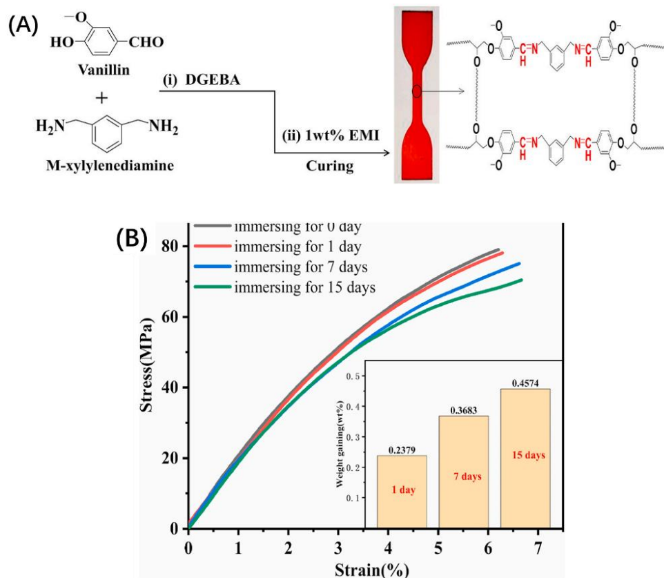
Figure 8: (A) Synthetic route of Van-EP bio-based vitrimer, (B) Typical stress-strain curves and weight gaining of Van-EP bio-based vitrimers after immersed in water for different times. Adapted with permission from ref. 93. Copyright 2020, Elsevier.
