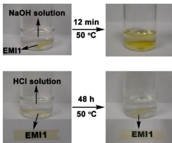
Figure 1: Appearance of EMI before and after immersing in 1 M NaOH aqueous solution (top) or 1 M HCl aqueous solution (bottom). Adapted with permission from ref. [65]. Copyright 2016 American Chemical Society.
