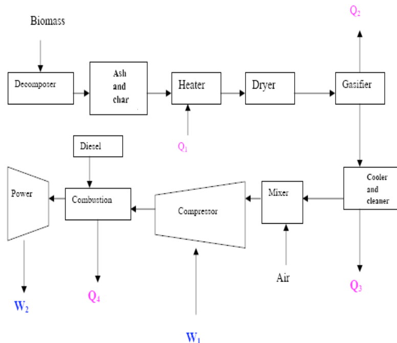
Figure 7: Advanced biomass power with diesel engine [11].
