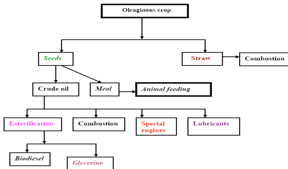
Figure 9: Flow chart of biodiesel production [11].
