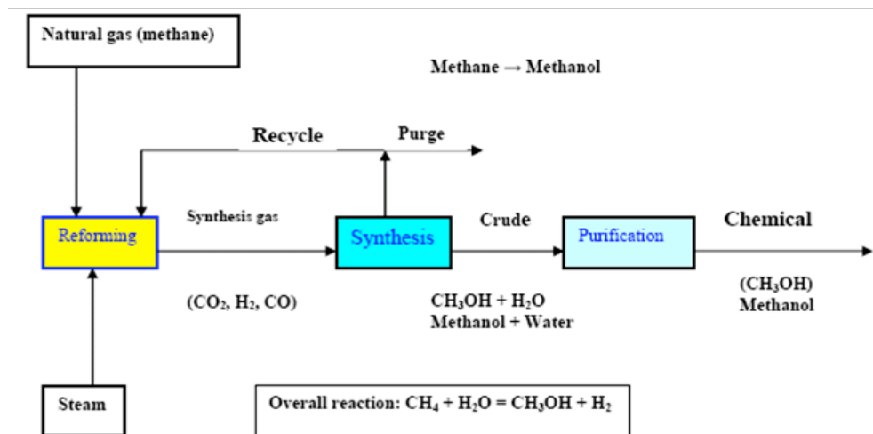
Figure 2: Schematic diagram shows methanol production [11].
