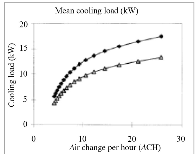
Figure 7: Cooling loads by night ventilation for desired room indoor air temperatures of 23 and 25°C [33].
