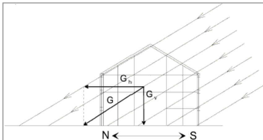
Figure 12: Relative horizontal and vertical components of solar radiation.
