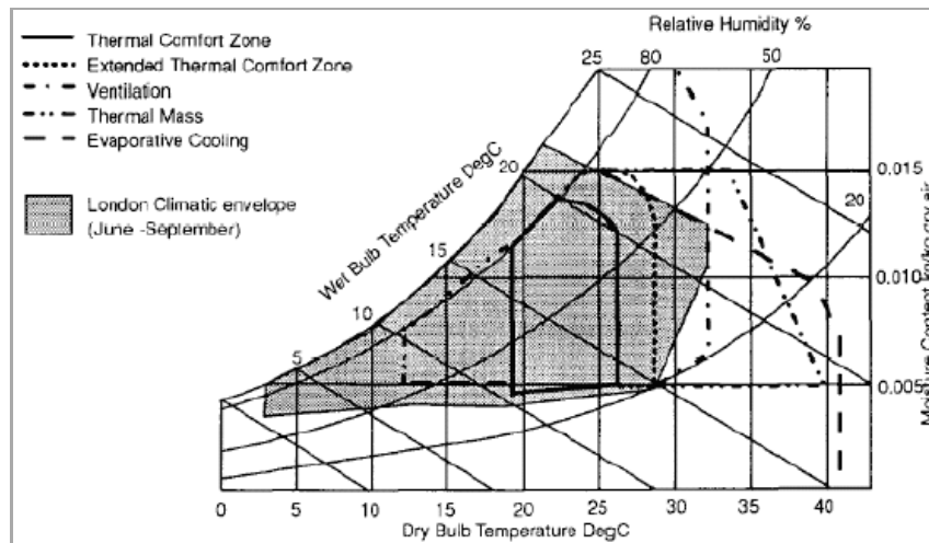
Figure 5: Bioclimatic chart with summer climatic envelope for London [32].
