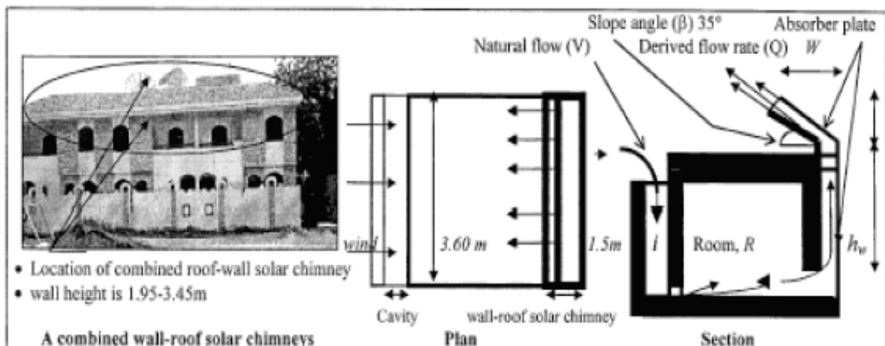
Figure 6: A combined wall-roof solar chimney incorporated into residential building Night ventilation [33].
