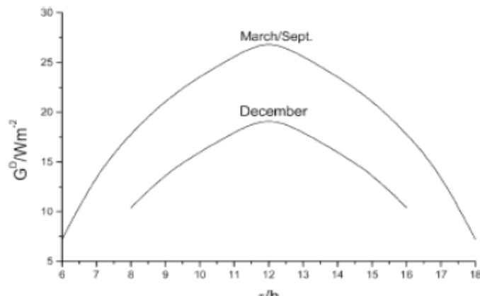
Figure 10: Ground irradiance from diffuse (sky) radiation from a clear sky at the shortest winter day and at equinox [38].
