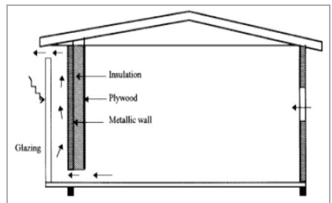
Figure 4: Schematic representations of the passive solar house and natural ventilation by metallic solar wall [28].
