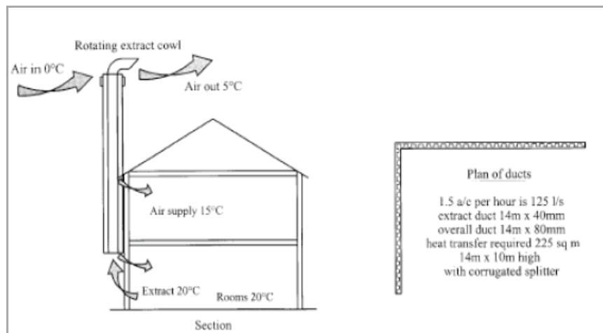
Figure 3: Ventilation duct supply and extract wraps around the building [27].
