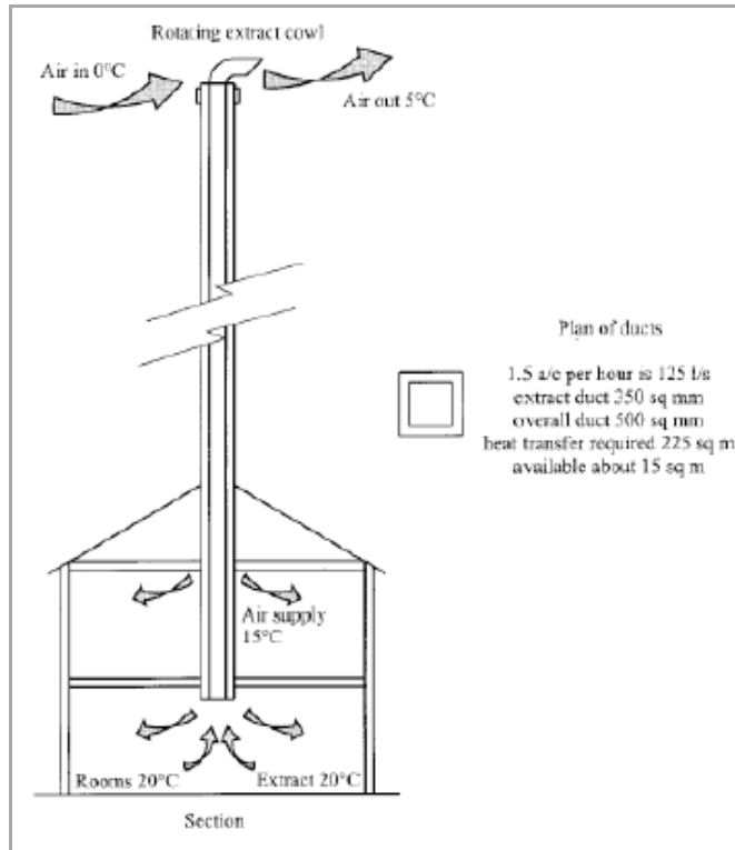
Figure 2: Small house natural ventilation with heat reclaims (A very tall chimney) [27].
