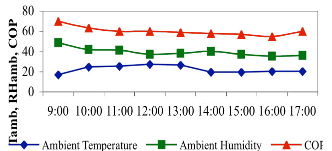
Figure 16: Ambient temperature, relative humidity and COP.
