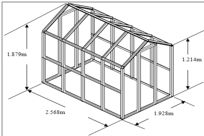
Figure 11: Greenhouse and base with horticultural glass [40].
